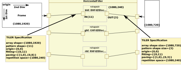
Figure 10. Downscaler tiler specification
